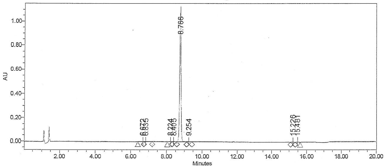
Auto-Scaled Chromatogram
